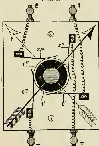
DIAGRAM OF COMMUTATOR.
